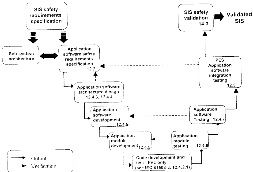
Figure 12 – Software development life cycle (the V-model)
